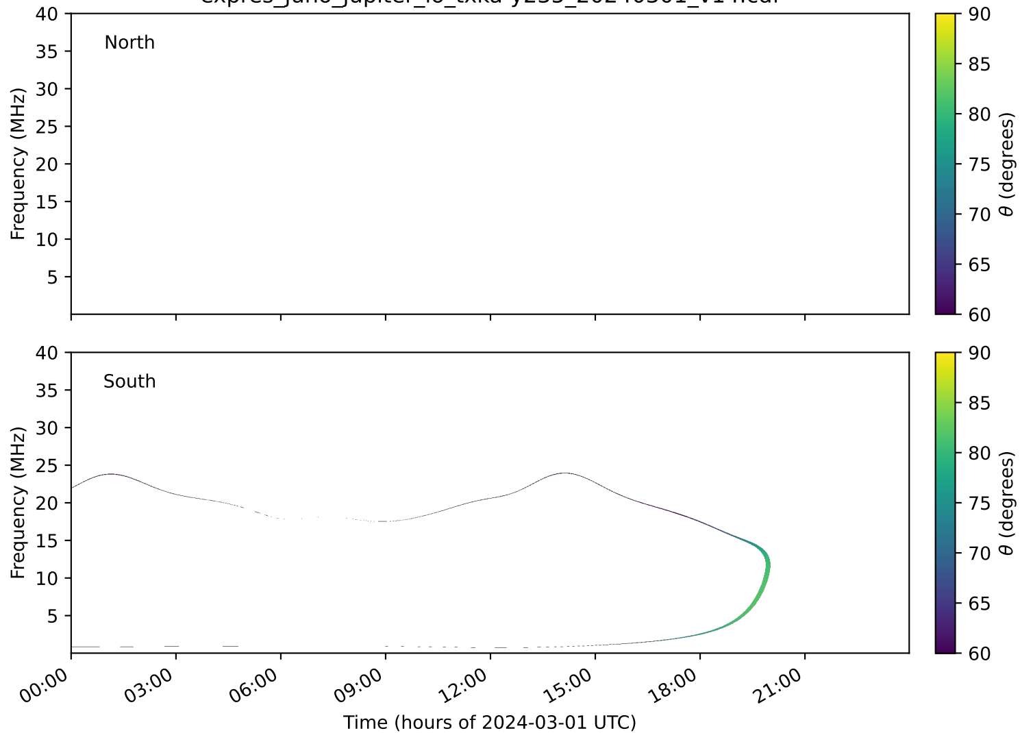
expres_juno_jupiter_io_txka-y235_20240301_v14.cdf
