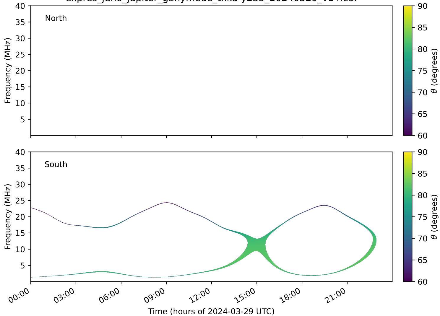
expres_juno_jupiter_ganymede_txka-y235_20240329_v14.cdf
