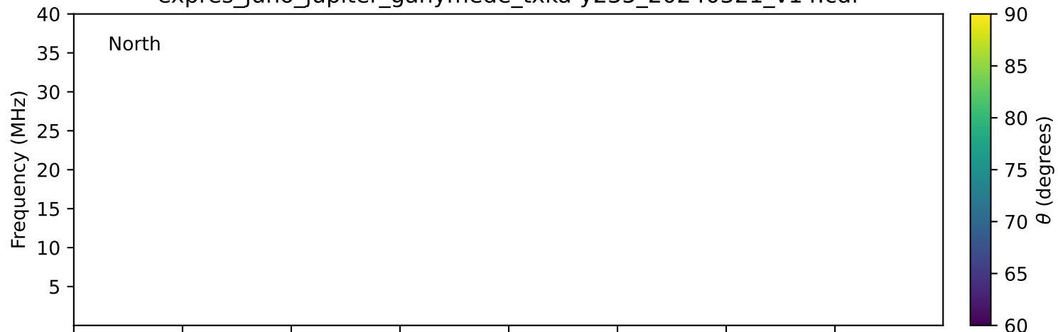
expres_juno_jupiter_ganymede_txka-y235_20240321_v14.cdf
