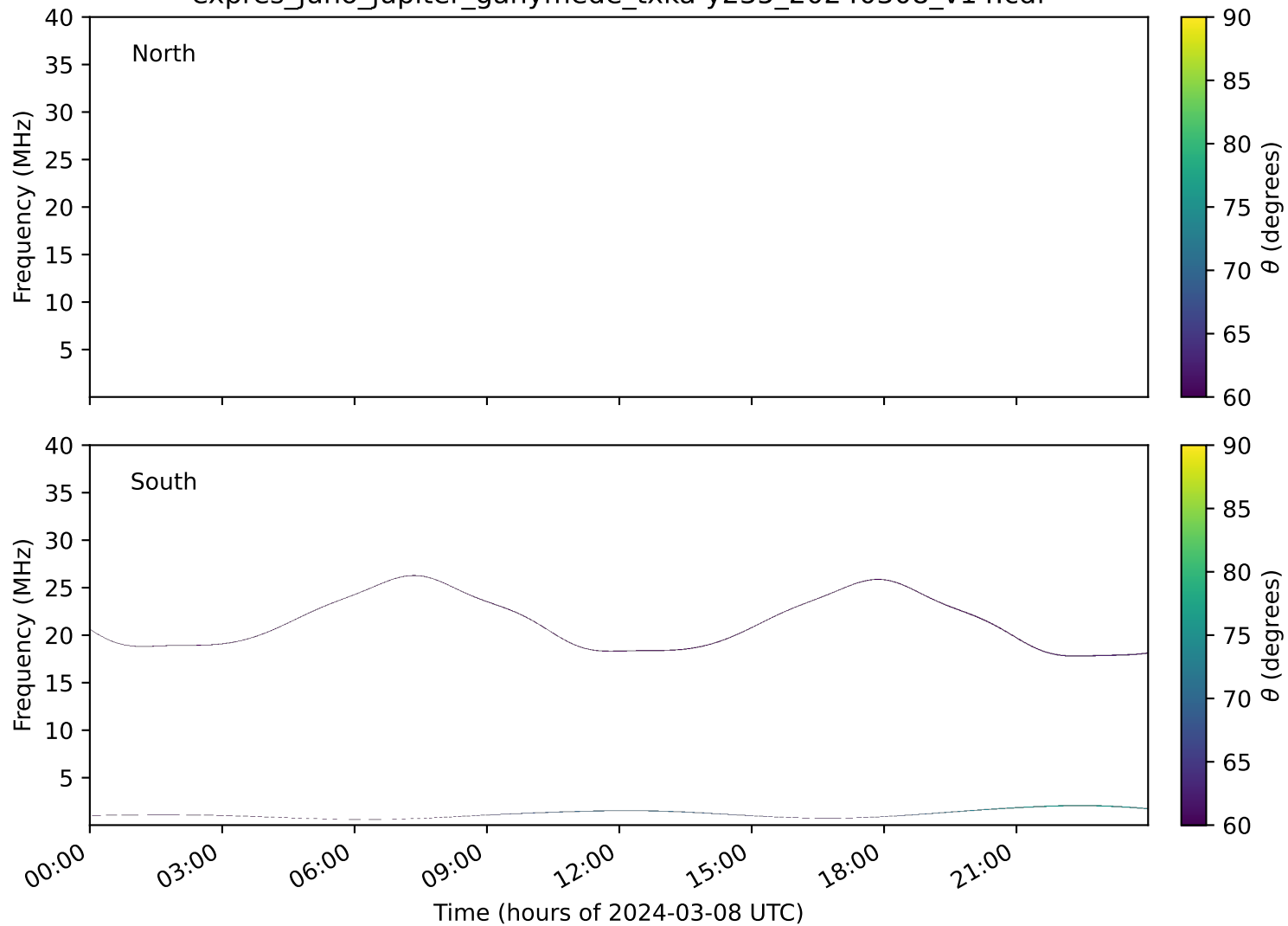
expres_juno_jupiter_ganymede_txka-y235_20240308_v14.cdf
