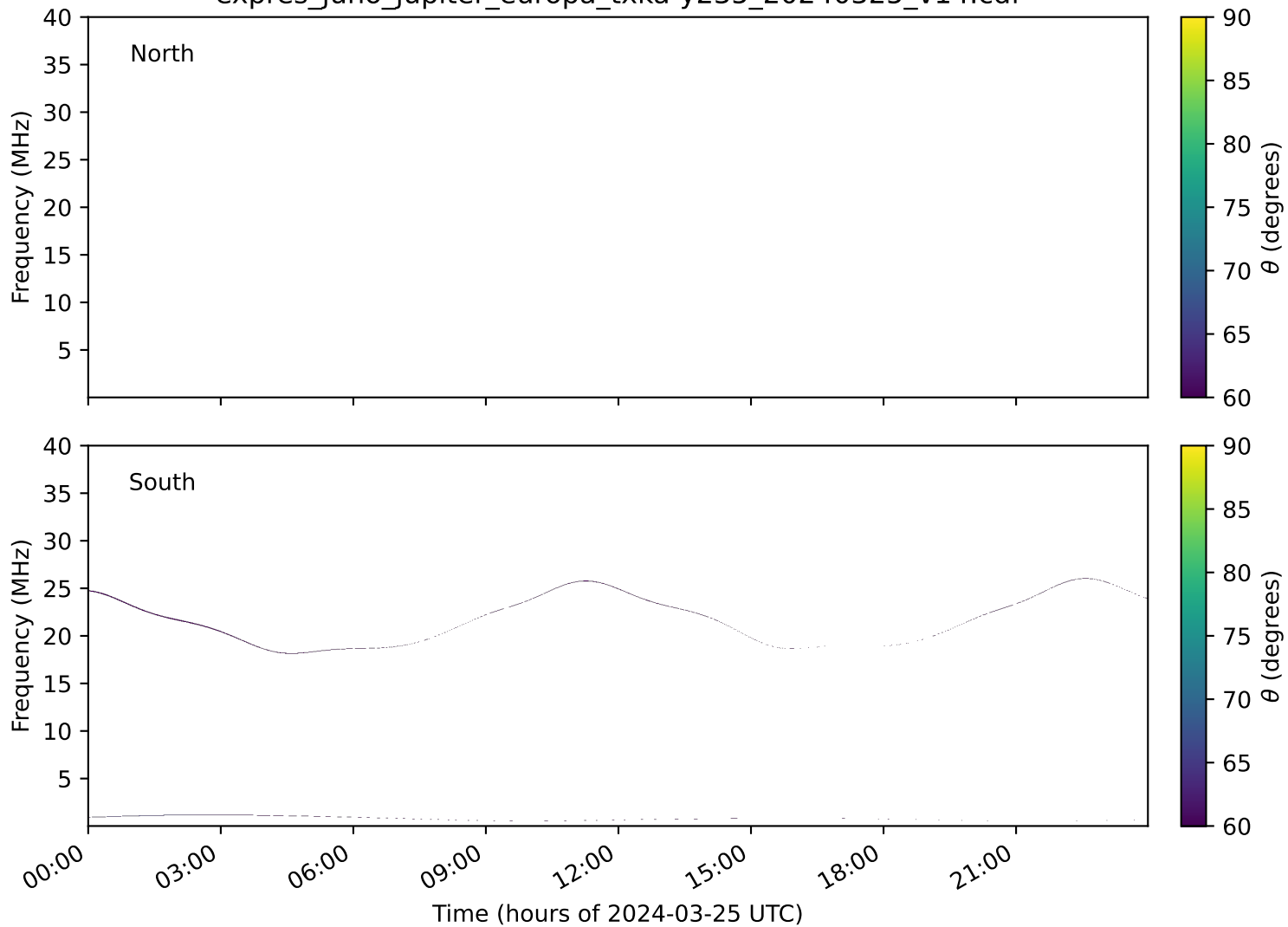
expres_juno_jupiter_europa_txka-y235_20240325_v14.cdf
