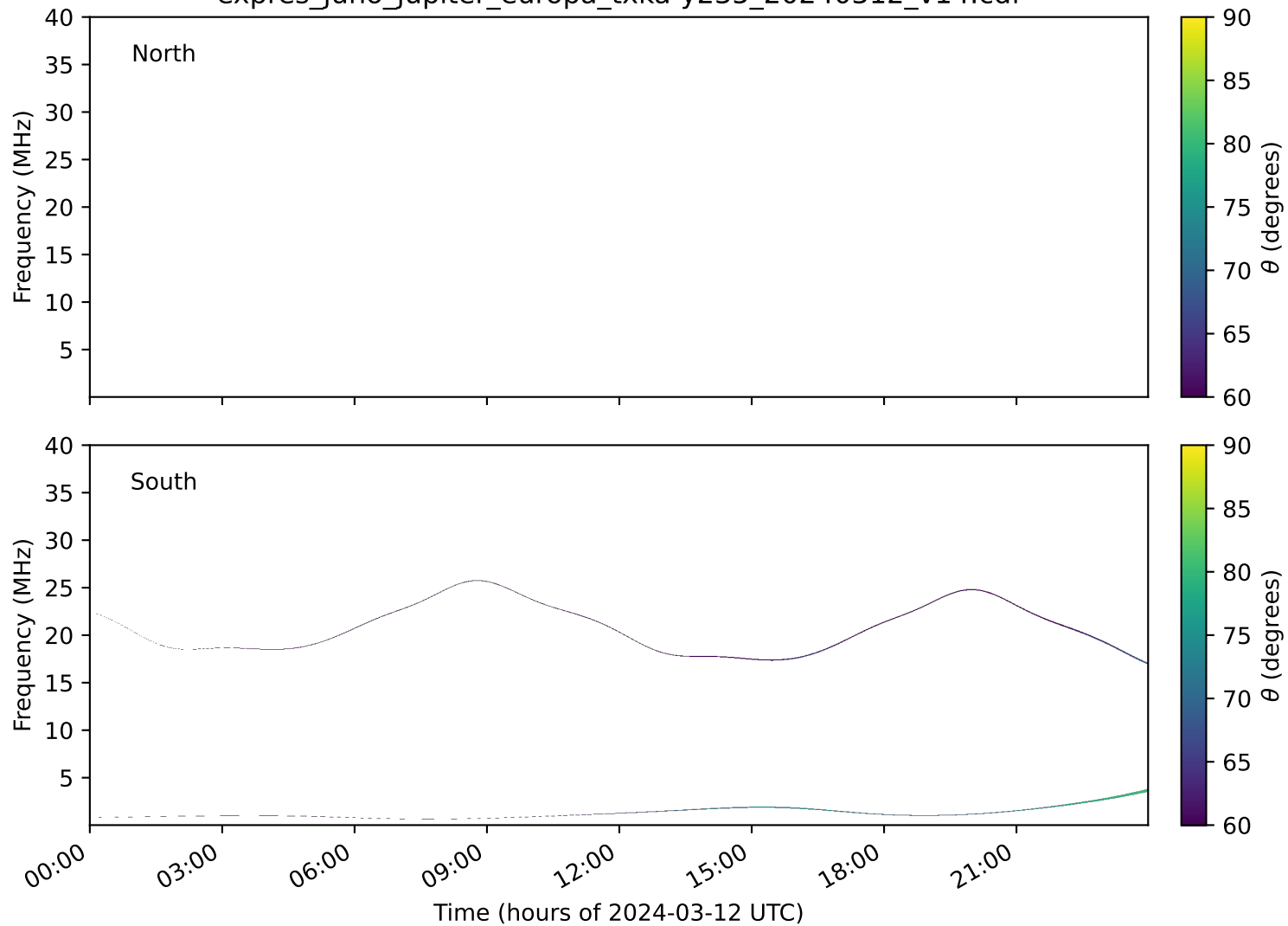
expres_juno_jupiter_europa_txka-y235_20240312_v14.cdf
