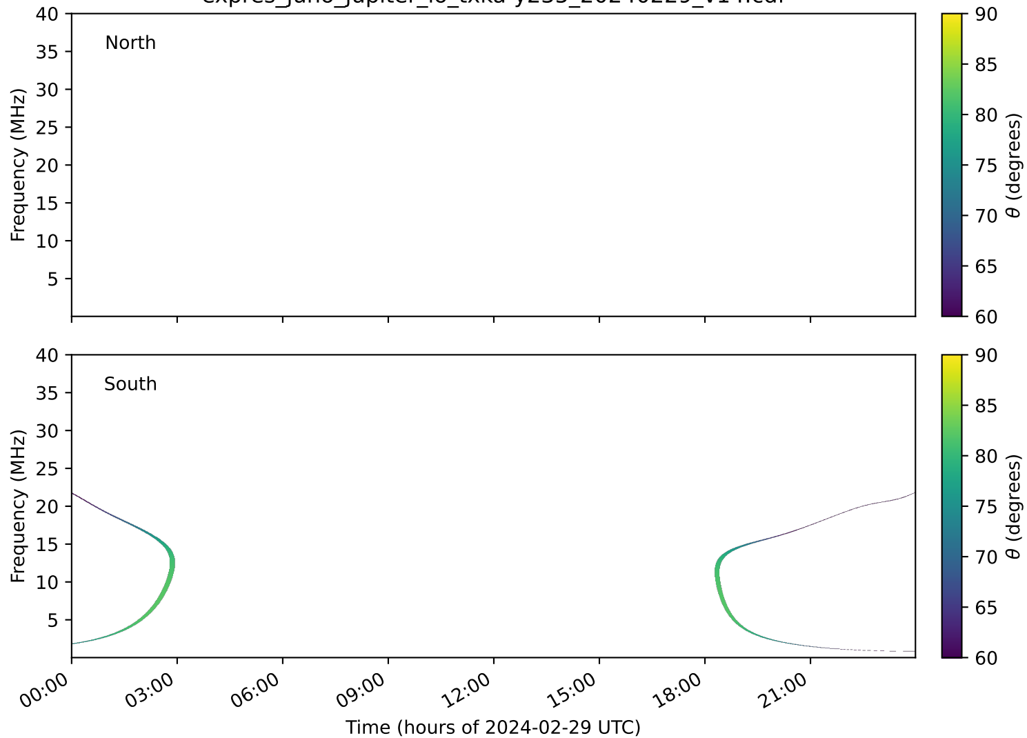
expres_juno_jupiter_io_txka-y235_20240229_v14.cdf
