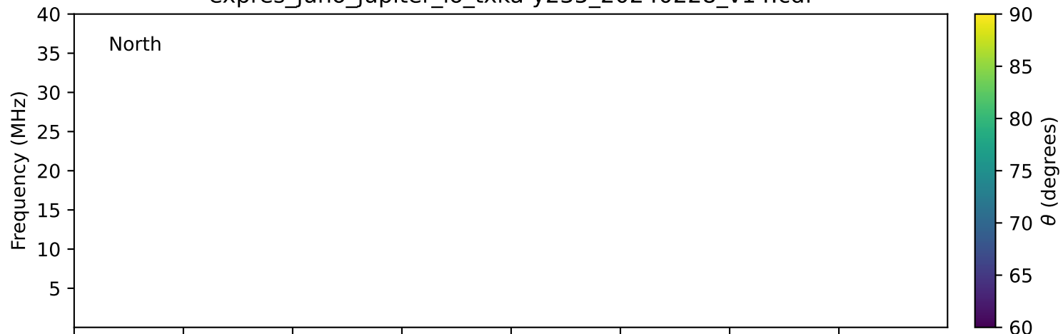
expres_juno_jupiter_io_txka-y235_20240228_v14.cdf
