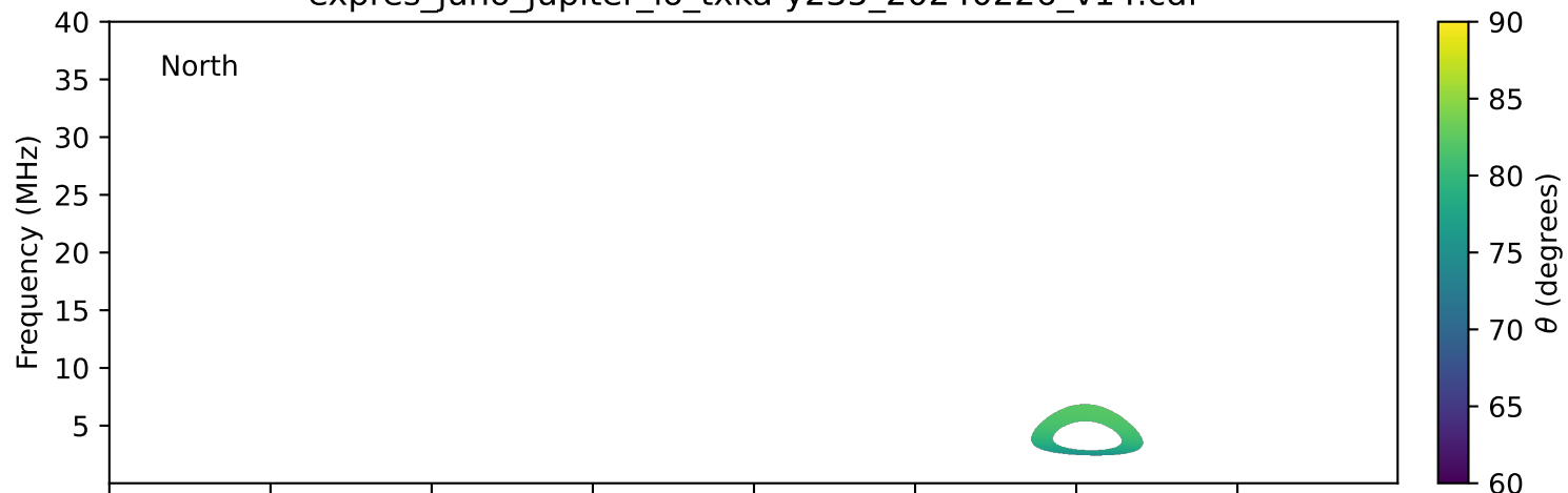
expres_juno_jupiter_io_txka-y235_20240226_v14.cdf
