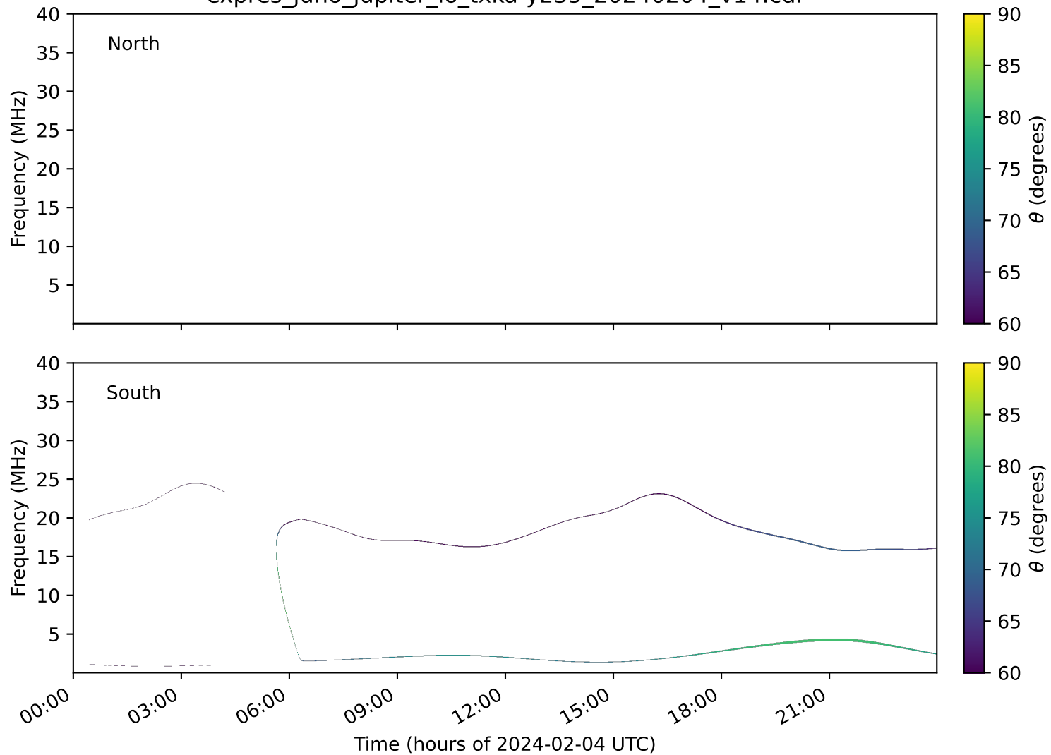
expres_juno_jupiter_io_txka-y235_20240204_v14.cdf
