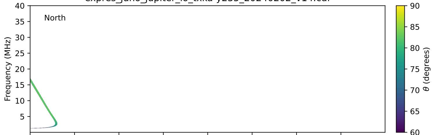
expres_juno_jupiter_io_txka-y235_20240202_v14.cdf
