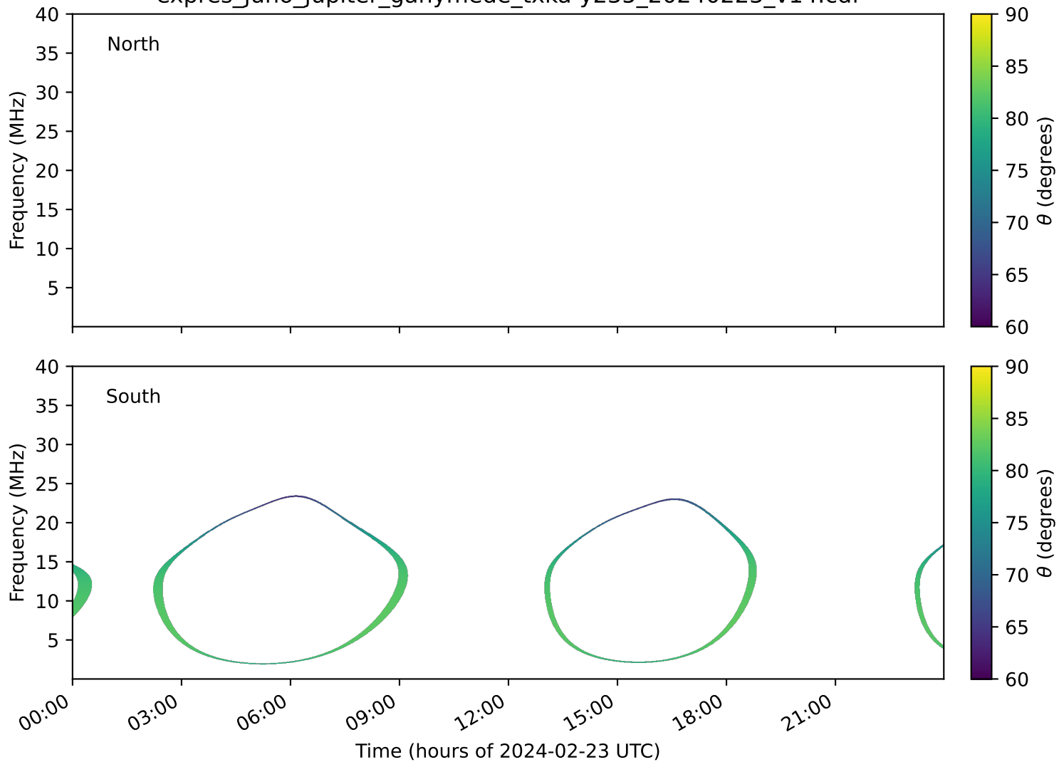
expres_juno_jupiter_ganymede_txka-y235_20240223_v14.cdf
