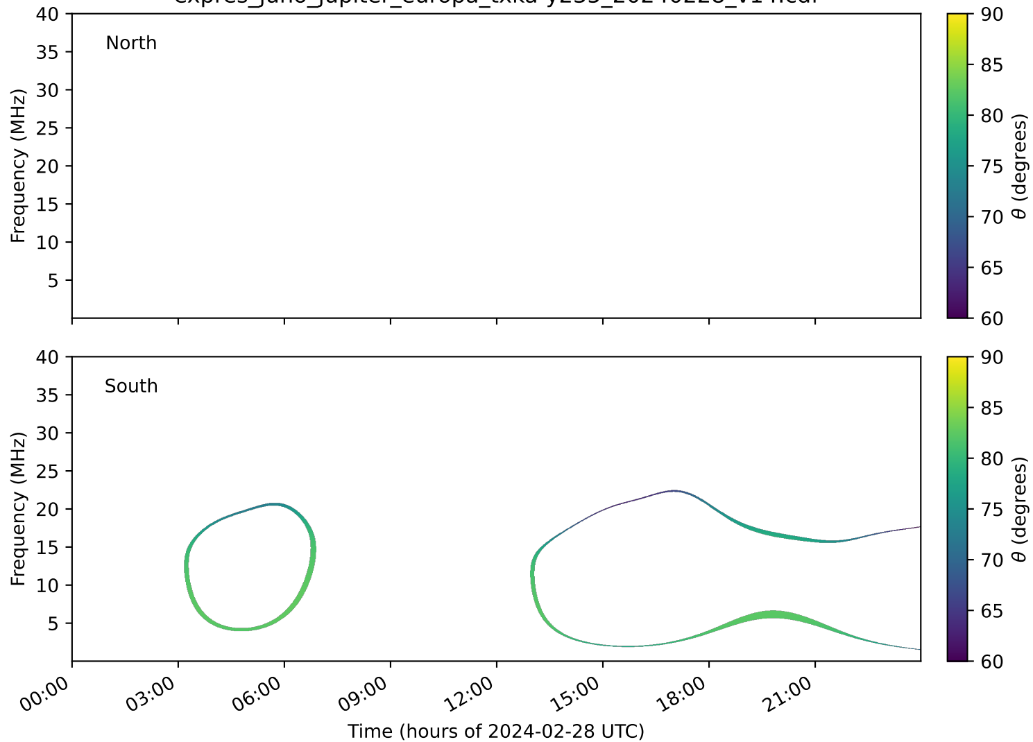
expres_juno_jupiter_europa_txka-y235_20240228_v14.cdf
