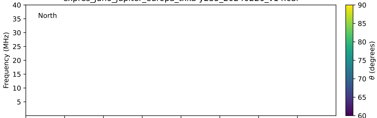
expres_juno_jupiter_europa_txka-y235_20240226_v14.cdf
