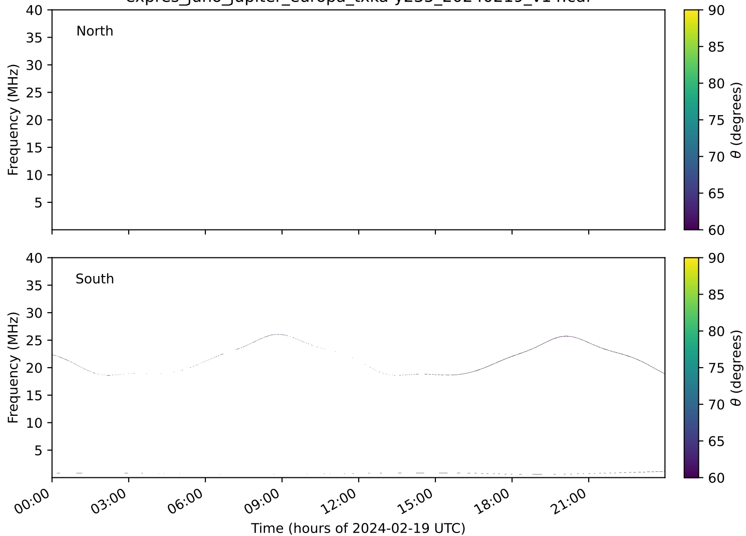
expres_juno_jupiter_europa_txka-y235_20240219_v14.cdf
