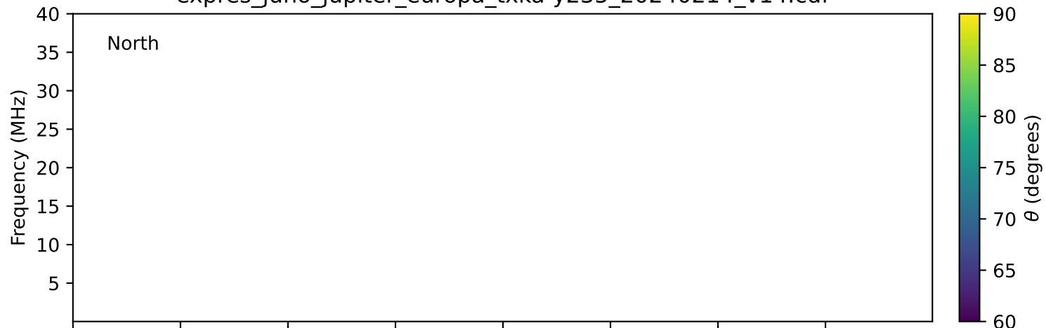
expres_juno_jupiter_europa_txka-y235_20240214_v14.cdf
