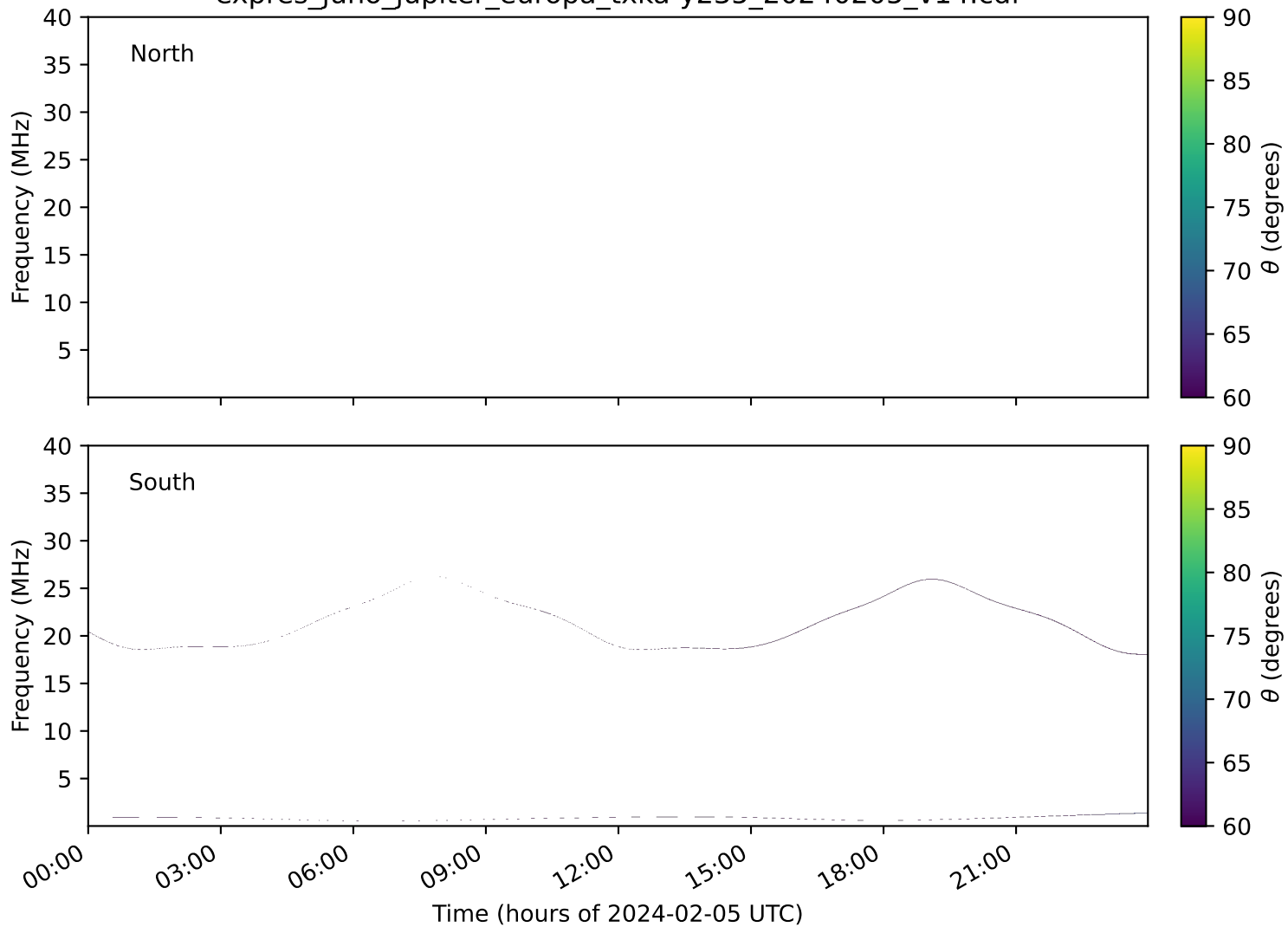
expres_juno_jupiter_europa_txka-y235_20240205_v14.cdf
