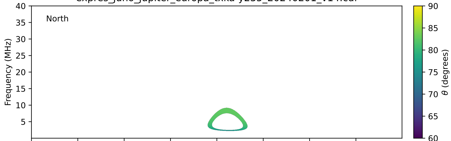
expres_juno_jupiter_europa_txka-y235_20240201_v14.cdf
