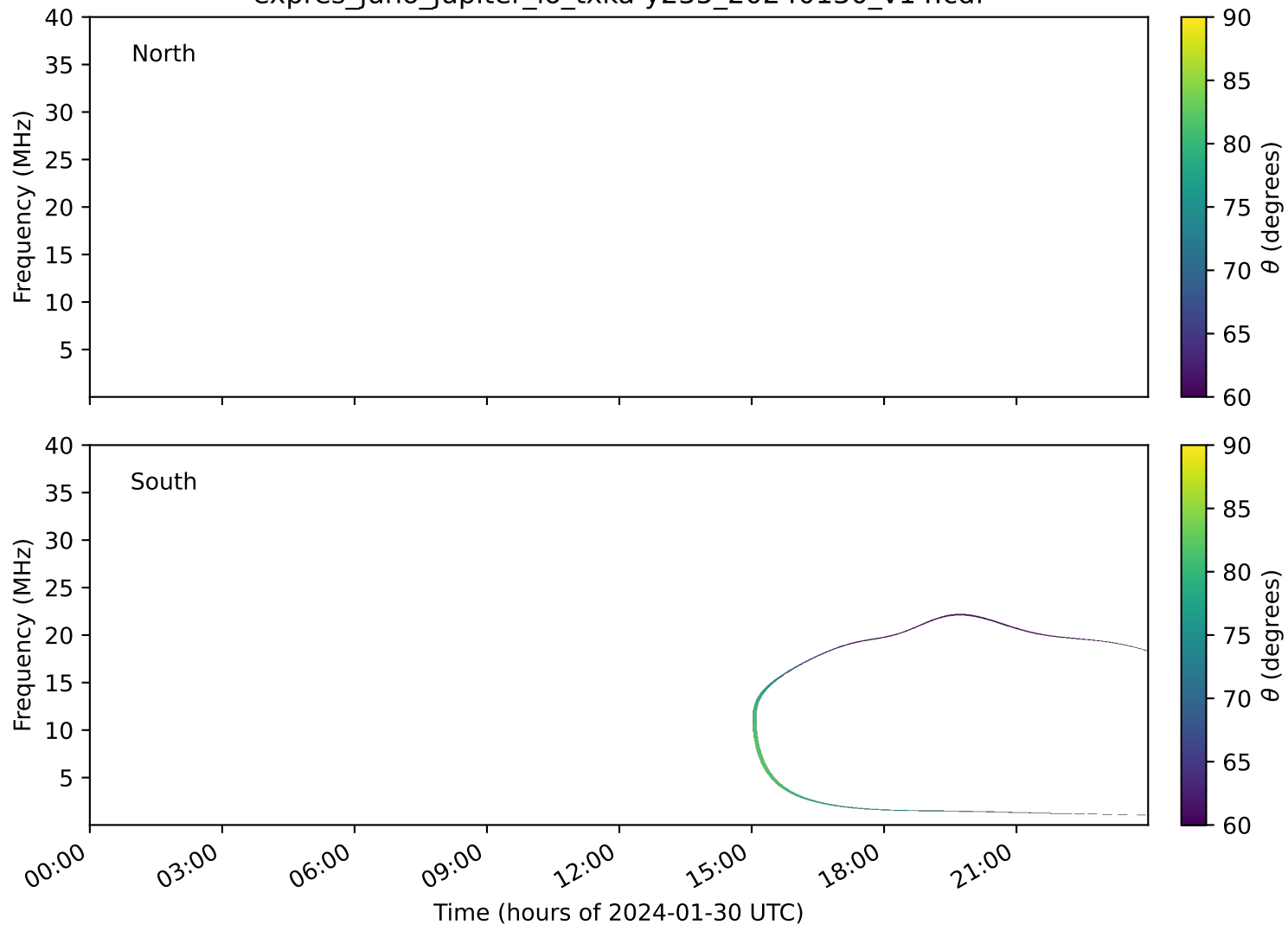
expres_juno_jupiter_io_txka-y235_20240130_v14.cdf
