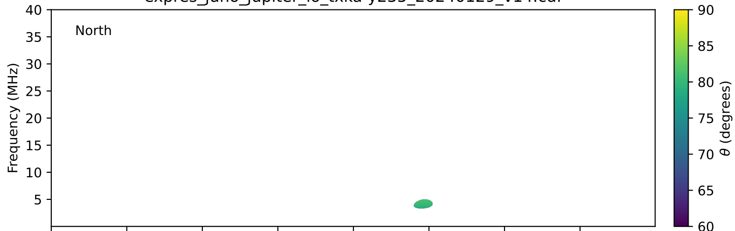
expres_juno_jupiter_io_txka-y235_20240129_v14.cdf
