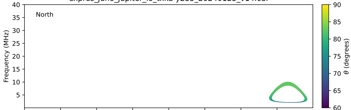
expres_juno_jupiter_io_txka-y235_20240125_v14.cdf
