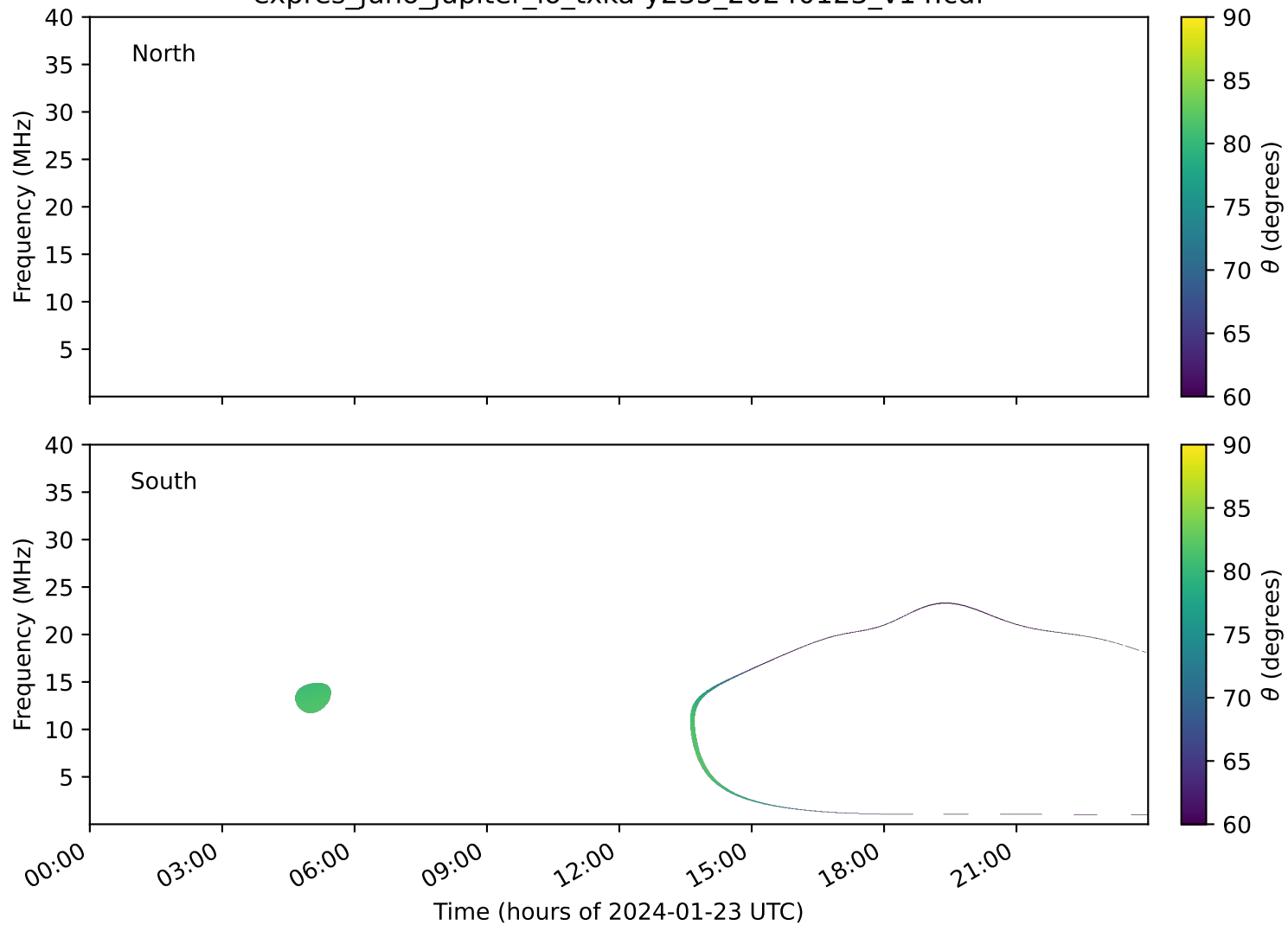
expres_juno_jupiter_io_txka-y235_20240123_v14.cdf
