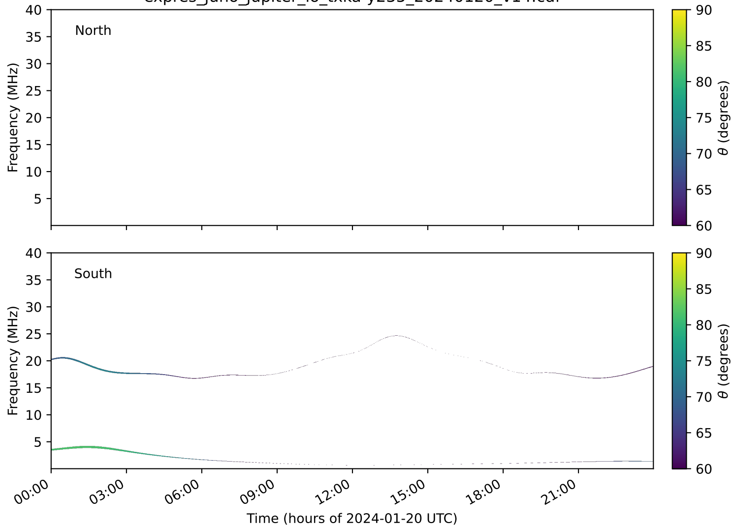
expres_juno_jupiter_io_txka-y235_20240120_v14.cdf
