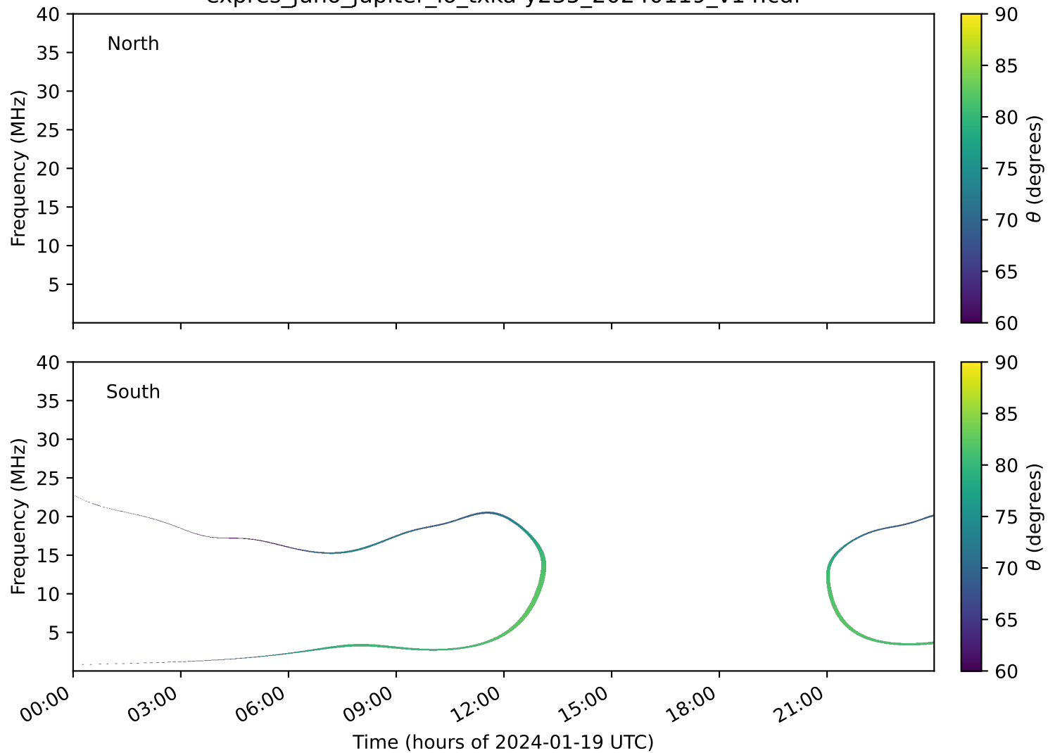
expres_juno_jupiter_io_txka-y235_20240119_v14.cdf
