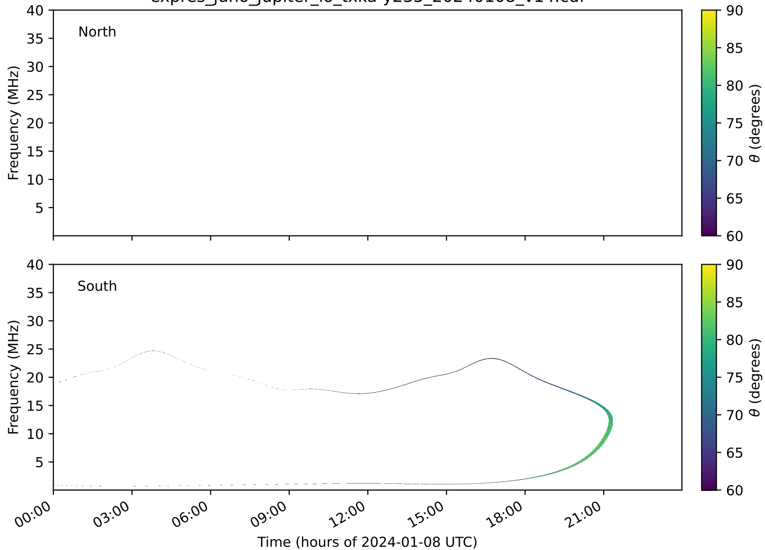
expres_juno_jupiter_io_txka-y235_20240108_v14.cdf
