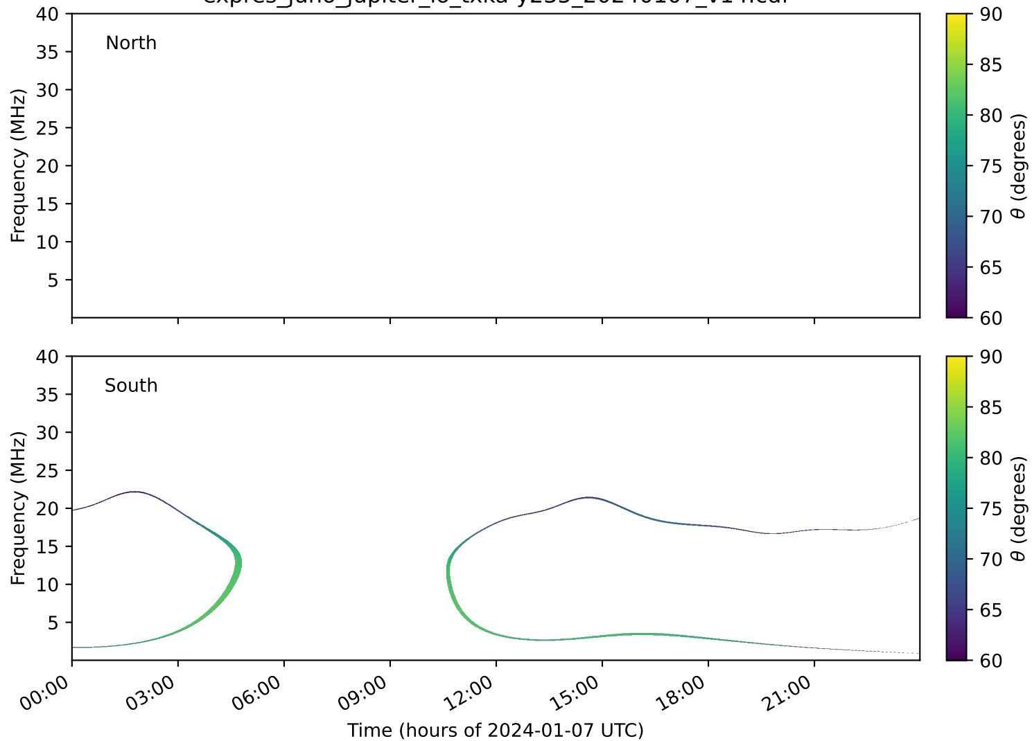
expres_juno_jupiter_io_txka-y235_20240107_v14.cdf
