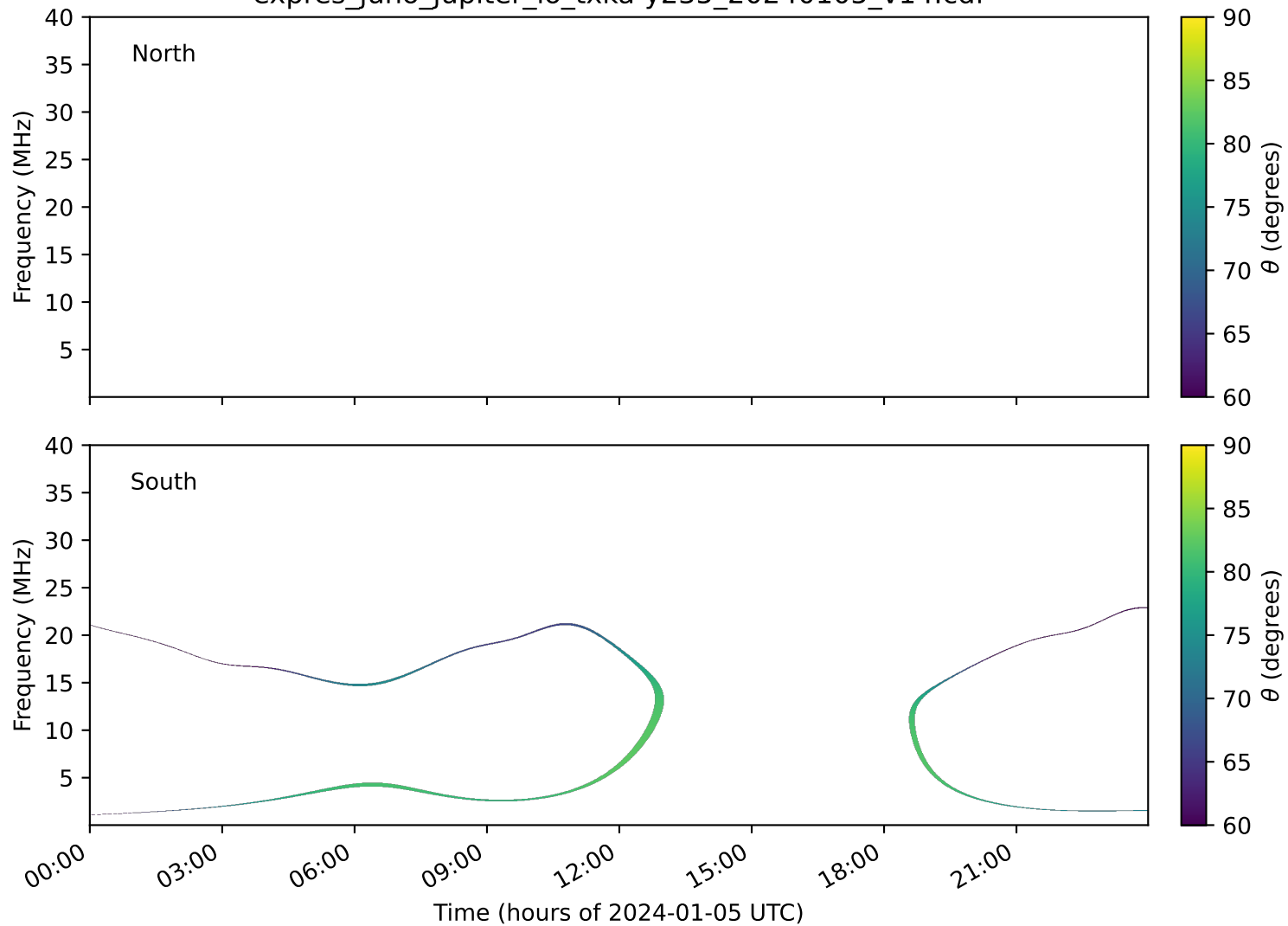
expres_juno_jupiter_io_txka-y235_20240105_v14.cdf
