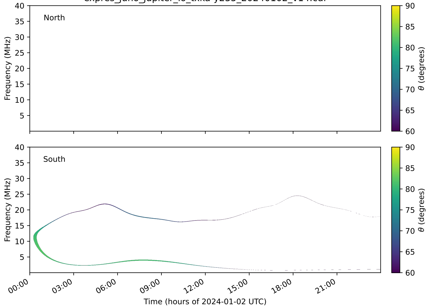
expres_juno_jupiter_io_txka-y235_20240102_v14.cdf
