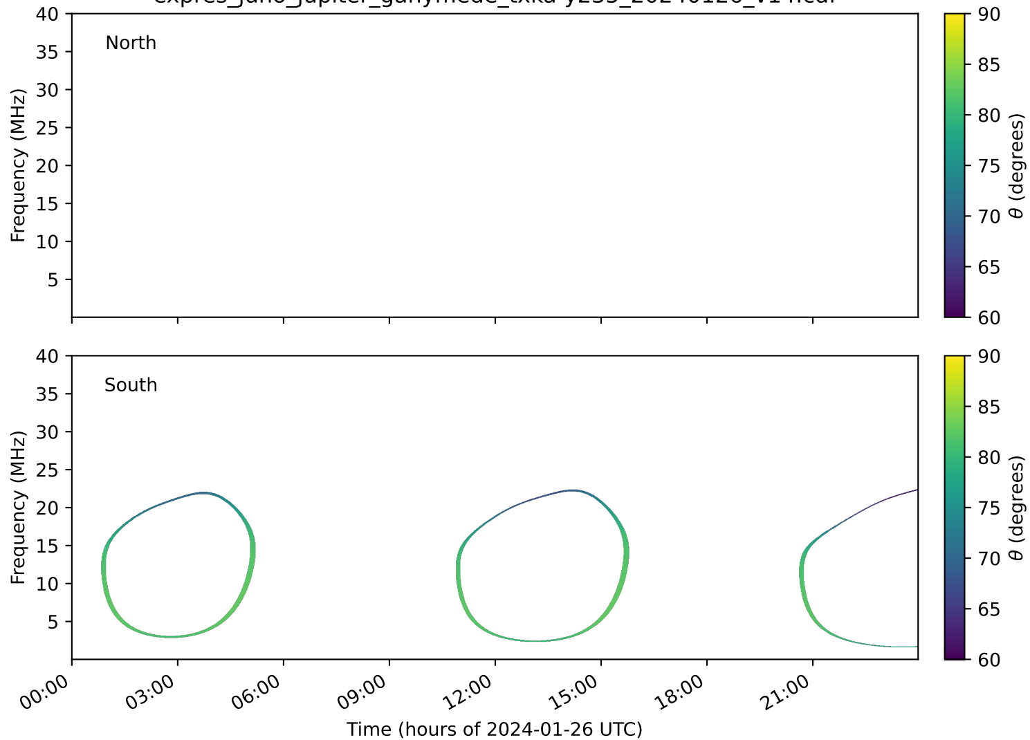
expres_juno_jupiter_ganymede_txka-y235_20240126_v14.cdf
