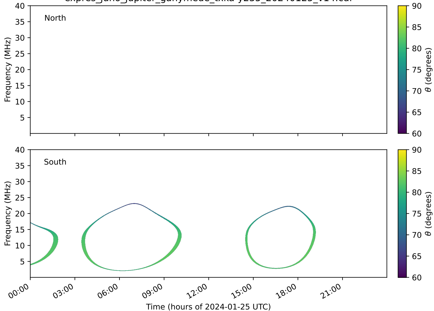
expres_juno_jupiter_ganymede_txka-y235_20240125_v14.cdf
