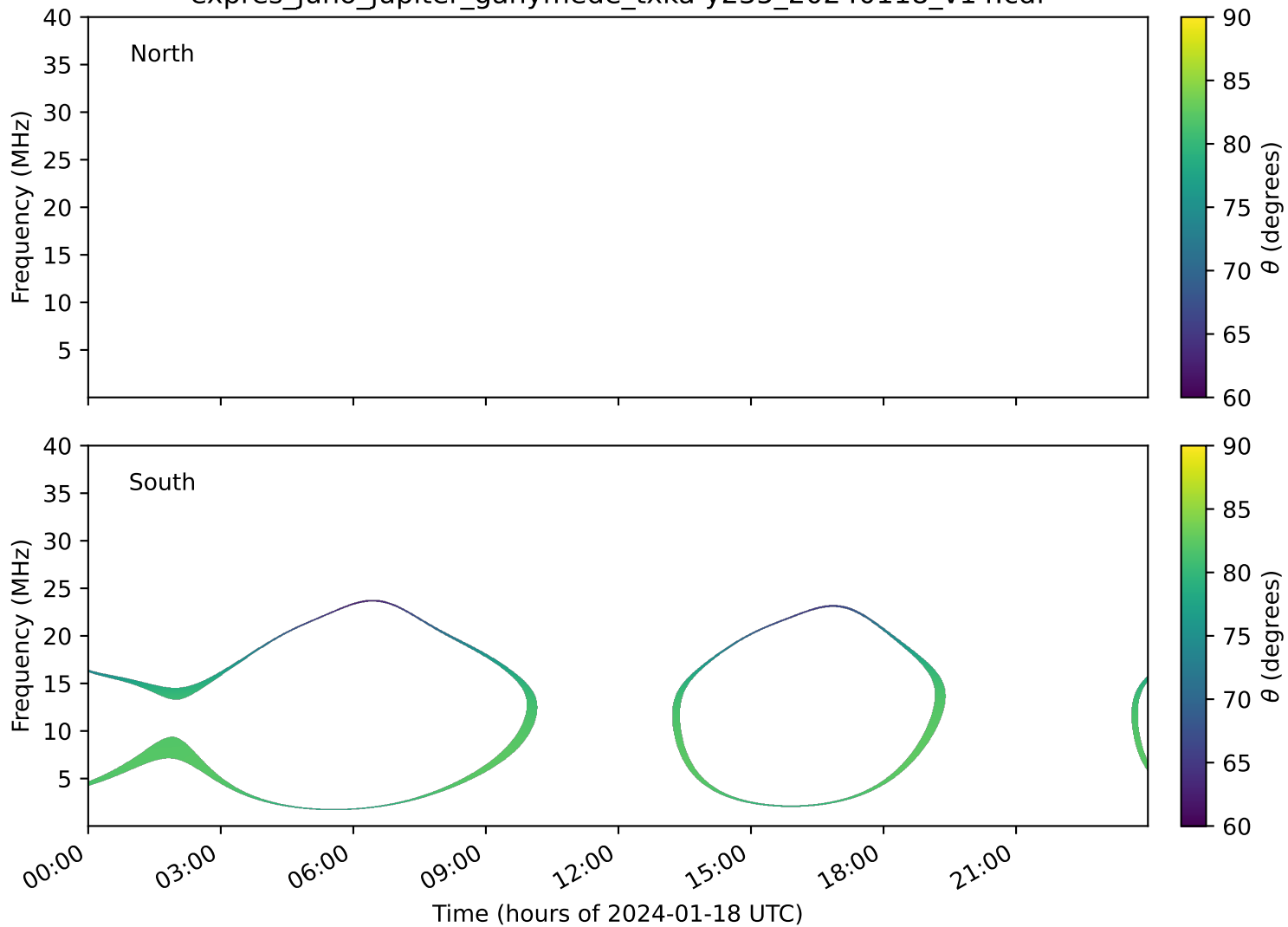
expres_juno_jupiter_ganymede_txka-y235_20240118_v14.cdf
