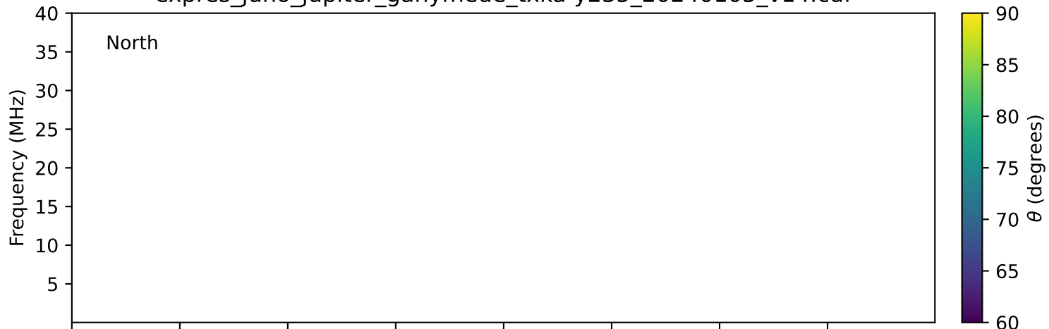
expres_juno_jupiter_ganymede_txka-y235_20240105_v14.cdf
