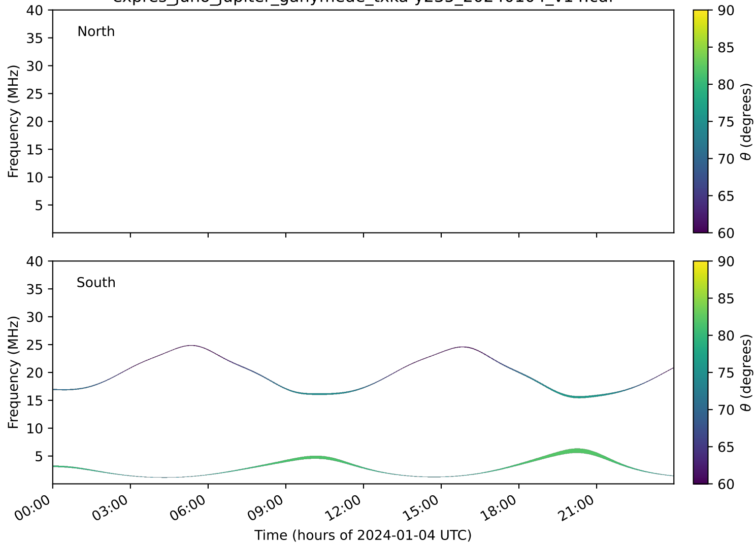
expres_juno_jupiter_ganymede_txka-y235_20240104_v14.cdf
