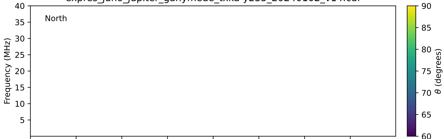
expres_juno_jupiter_ganymede_txka-y235_20240102_v14.cdf
