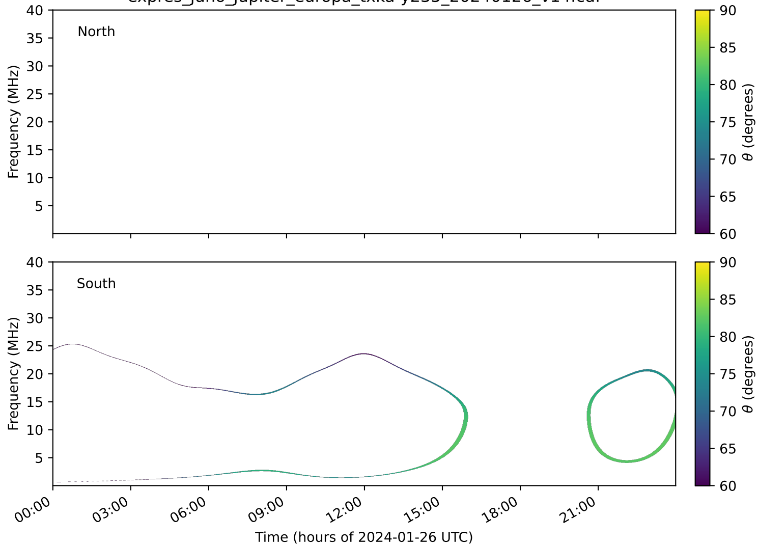
expres_juno_jupiter_europa_txka-y235_20240126_v14.cdf
