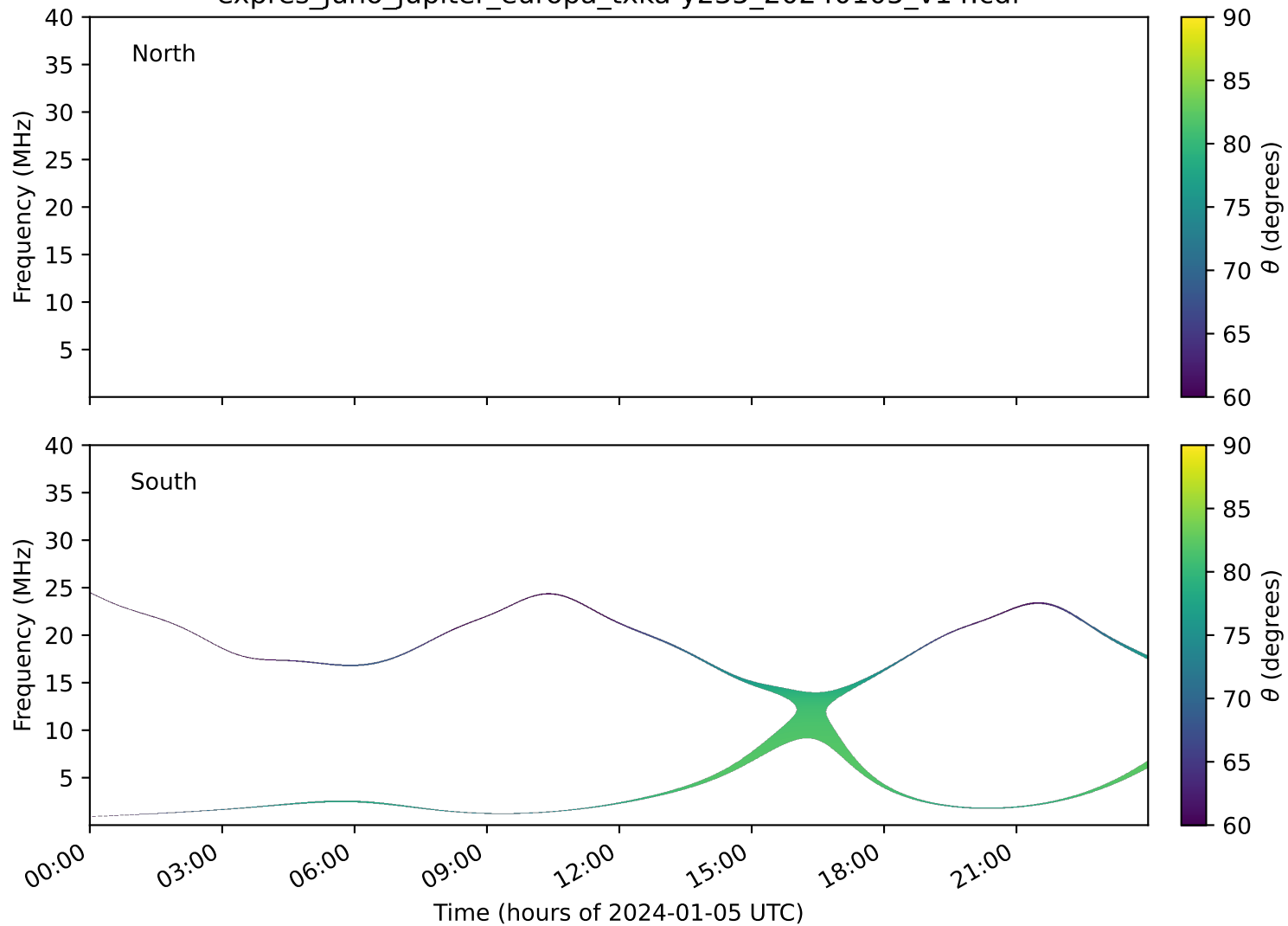
expres_juno_jupiter_europa_txka-y235_20240105_v14.cdf
