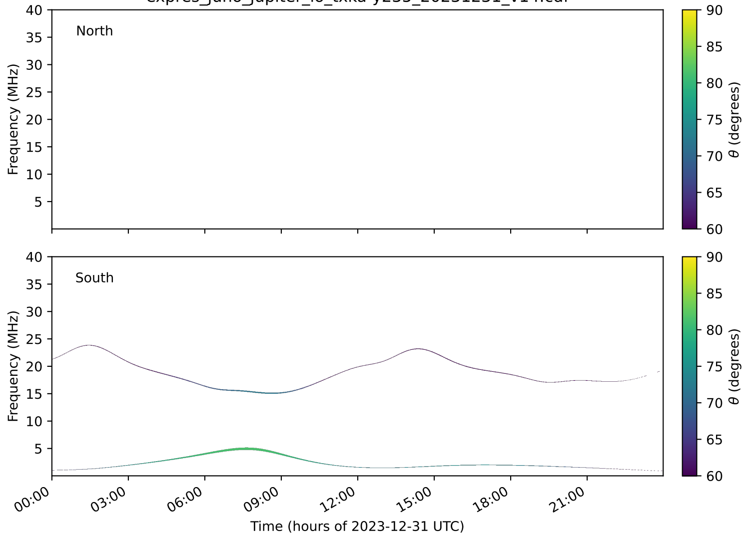
expres_juno_jupiter_io_txka-y235_20231231_v14.cdf
