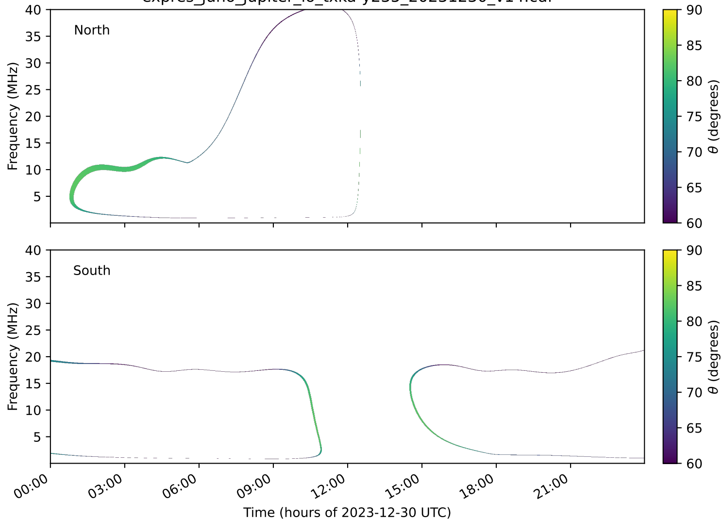
expres_juno_jupiter_io_txka-y235_20231230_v14.cdf
