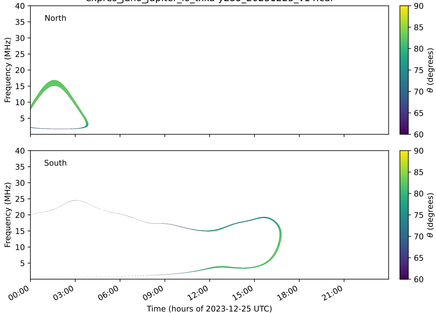
expres_juno_jupiter_io_txka-y235_20231225_v14.cdf
