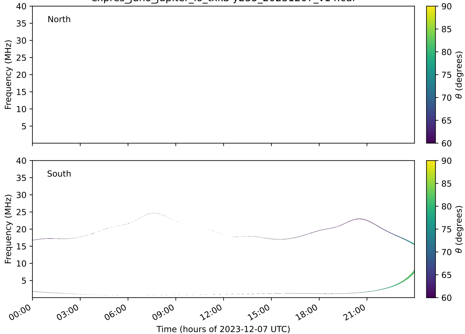
expres_juno_jupiter_io_txka-y235_20231207_v14.cdf
