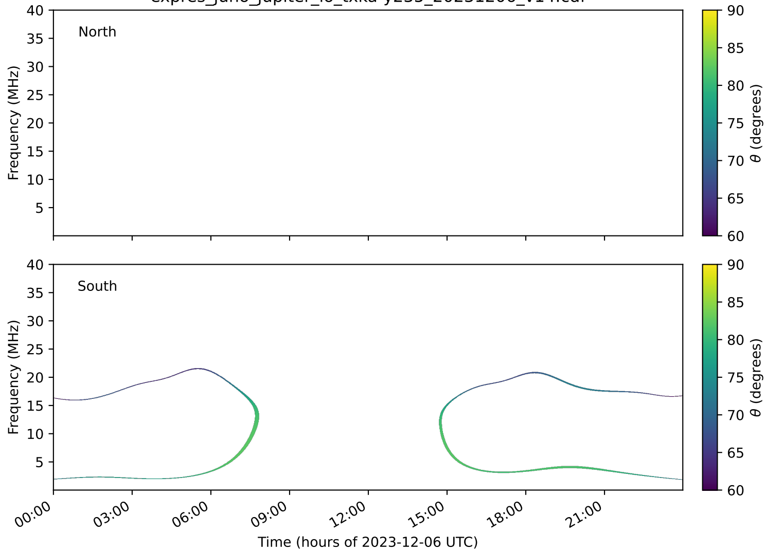
expres_juno_jupiter_io_txka-y235_20231206_v14.cdf
