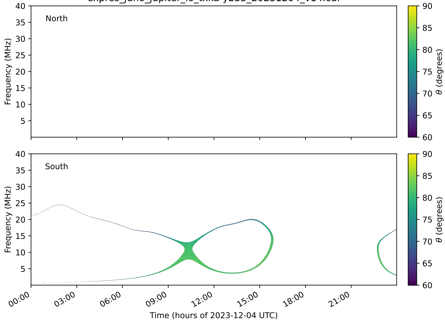
expres_juno_jupiter_io_txka-y235_20231204_v14.cdf
