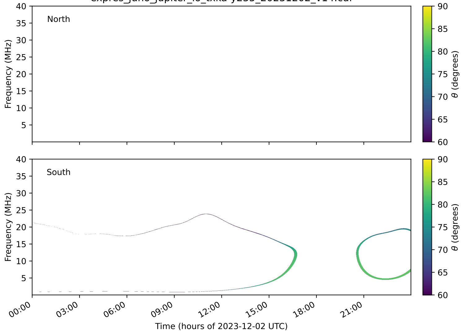
expres_juno_jupiter_io_txka-y235_20231202_v14.cdf
