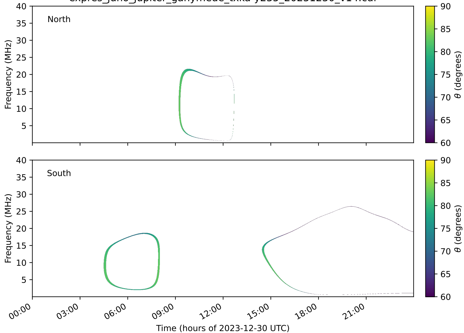
expres_juno_jupiter_ganymede_txka-y235_20231230_v14.cdf
