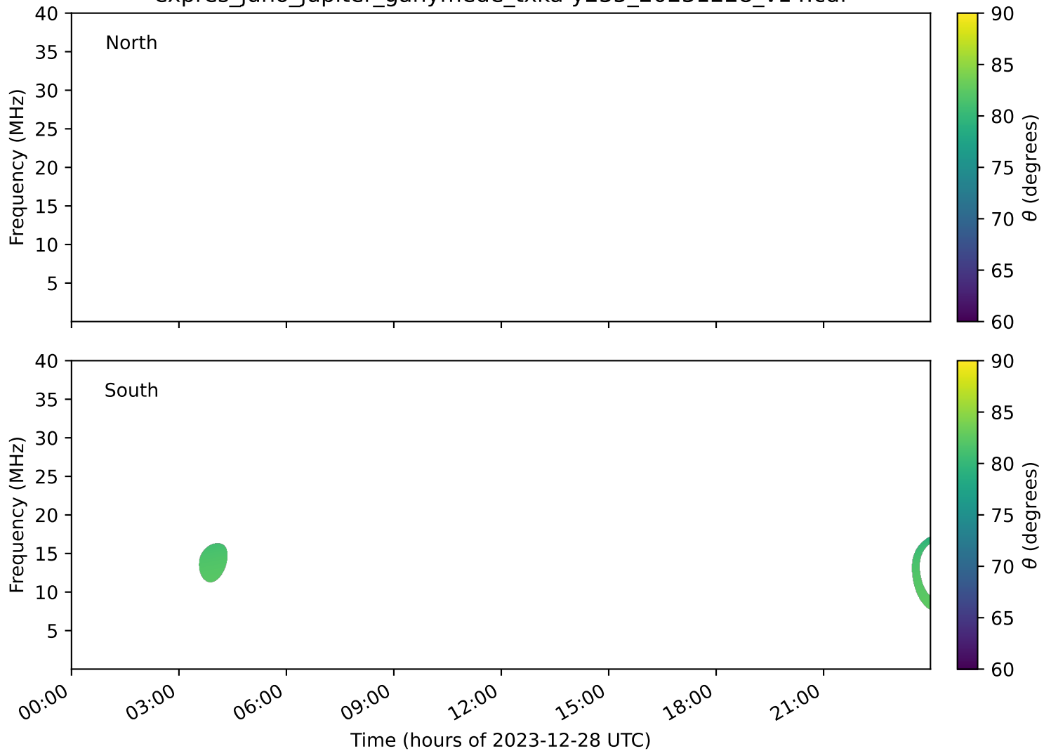
expres_juno_jupiter_ganymede_txka-y235_20231228_v14.cdf
