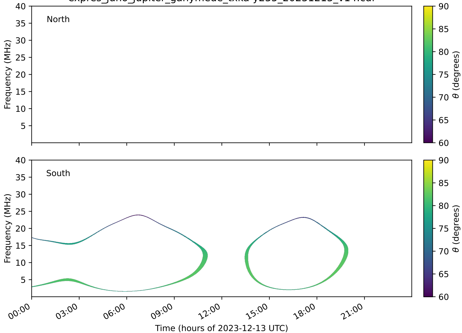
expres_juno_jupiter_ganymede_txka-y235_20231213_v14.cdf
