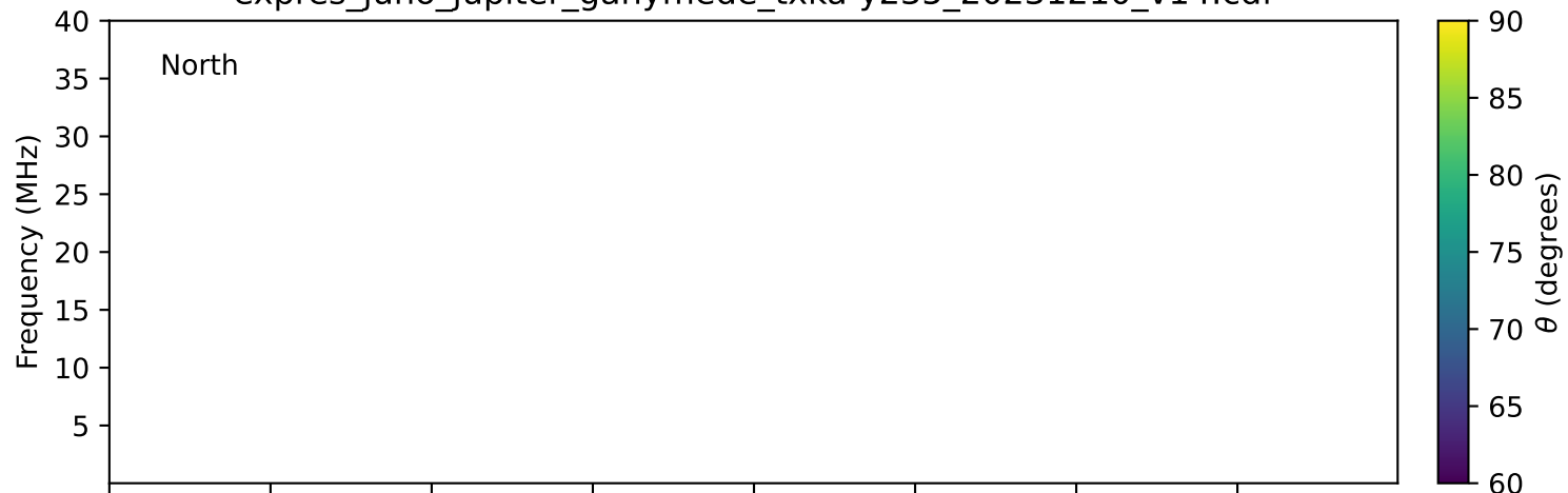
expres_juno_jupiter_ganymede_txka-y235_20231210_v14.cdf
