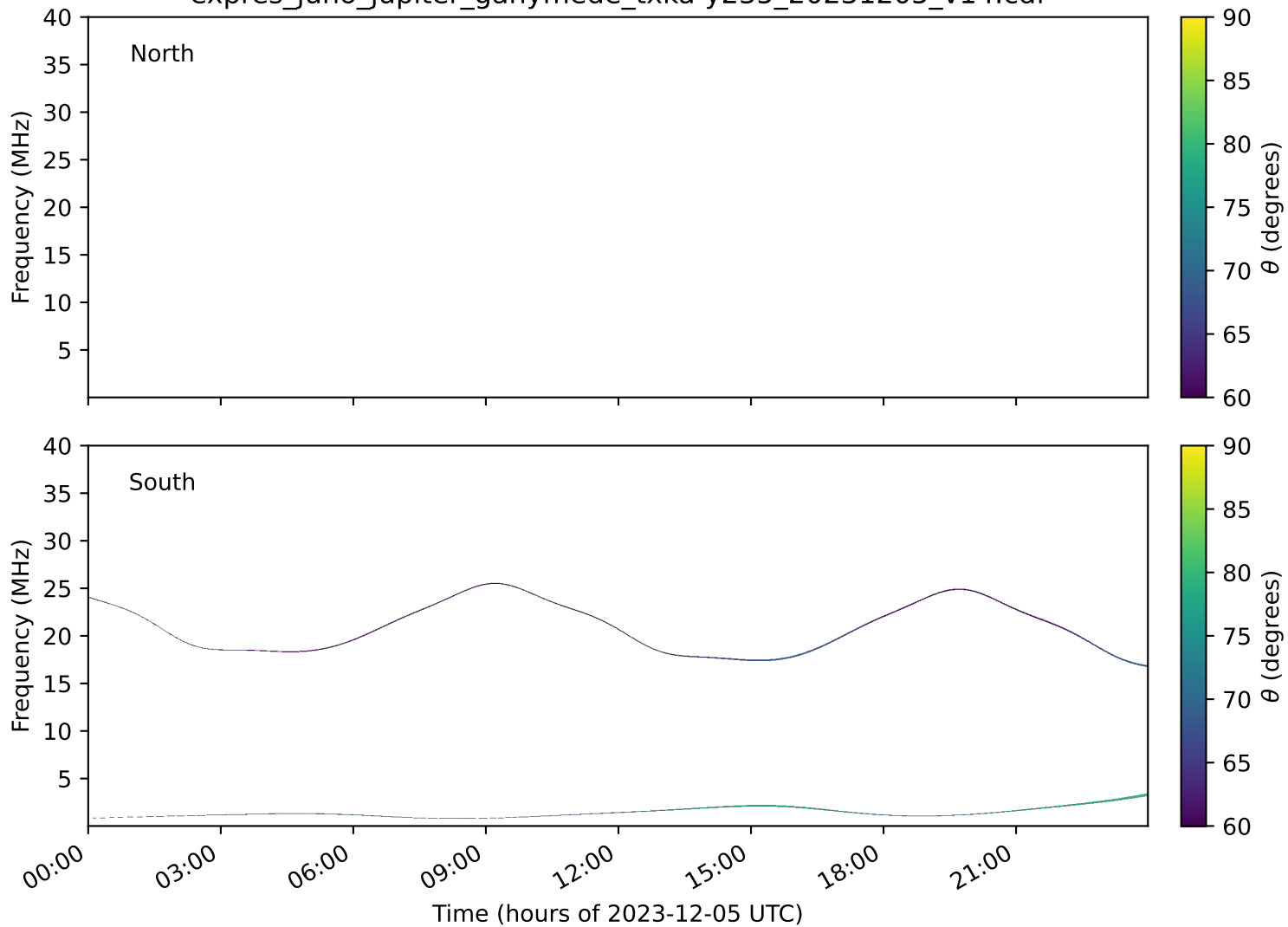
expres_juno_jupiter_ganymede_txka-y235_20231205_v14.cdf
