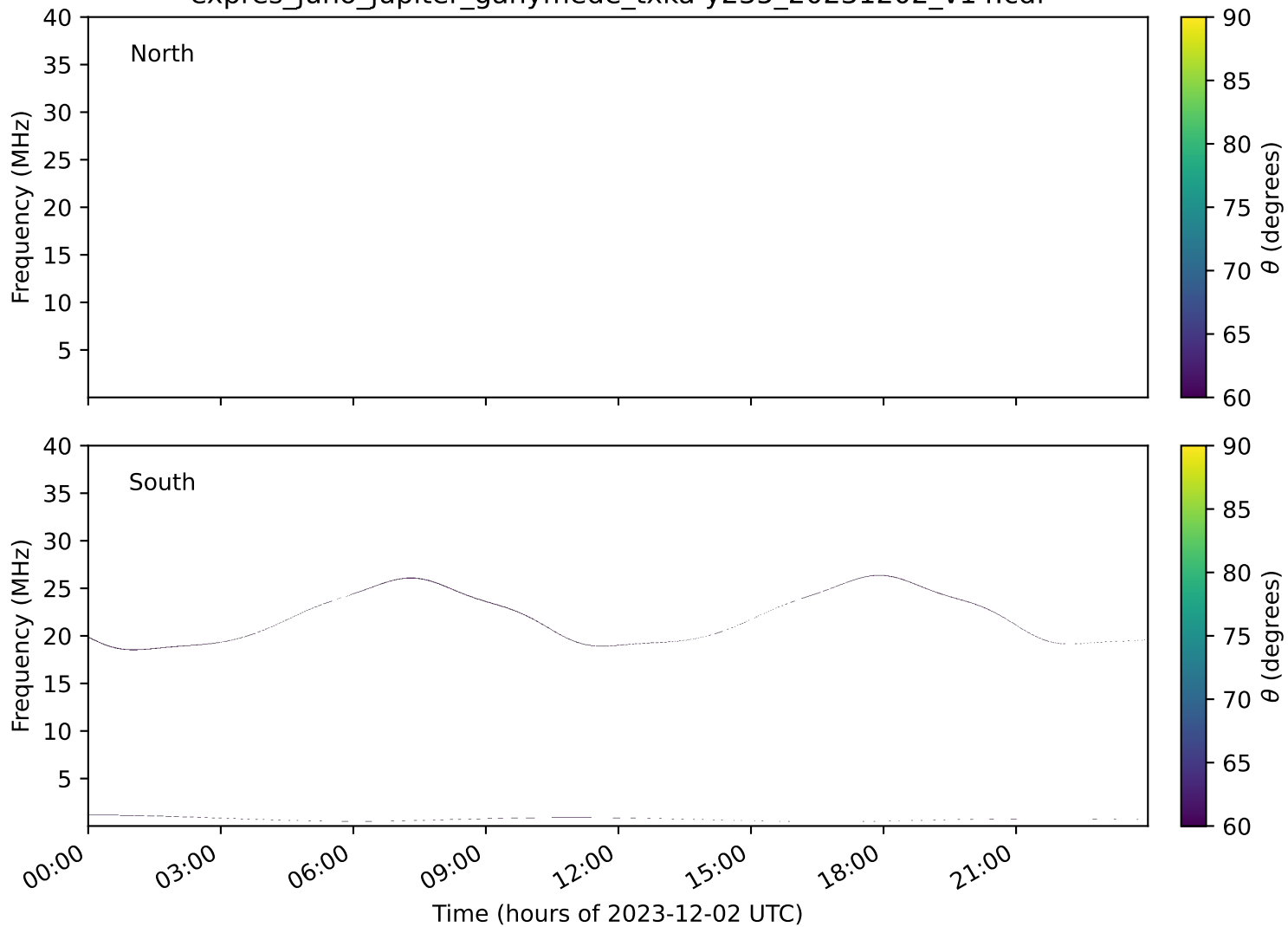
expres_juno_jupiter_ganymede_txka-y235_20231202_v14.cdf
