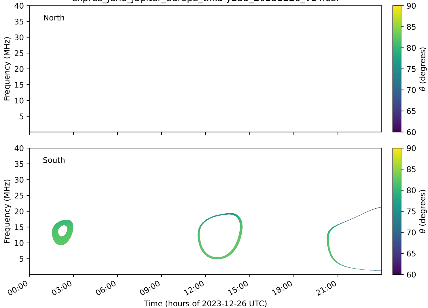
expres_juno_jupiter_europa_txka-y235_20231226_v14.cdf
